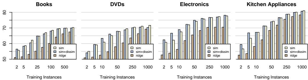
Figure 2: Accuracy of feature network regularization on the sentiment datasets feature classes and dissimilarity edges to regularize the small sent of SentiWordNet features.
